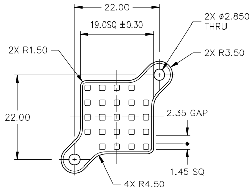
SR19-XXBC FOR Ø2.500 ± 0.05 PCB HOLES
