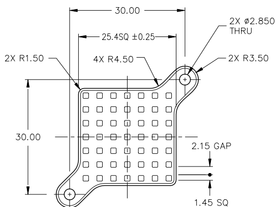
SR25-XXBC FOR Ø2.500 ±0.05 PCB HOLES
