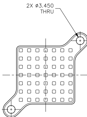
SR25-XXB FOR Ø3.175 ±0.05 PCB HOLES
