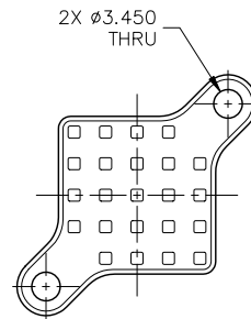
SR19-XXB FOR Ø3.175 ± 0.05 PCB HOLES
